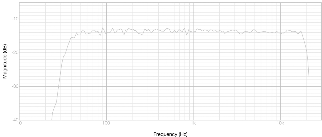
Frequency Response (1/24 Octave Smoothing)
